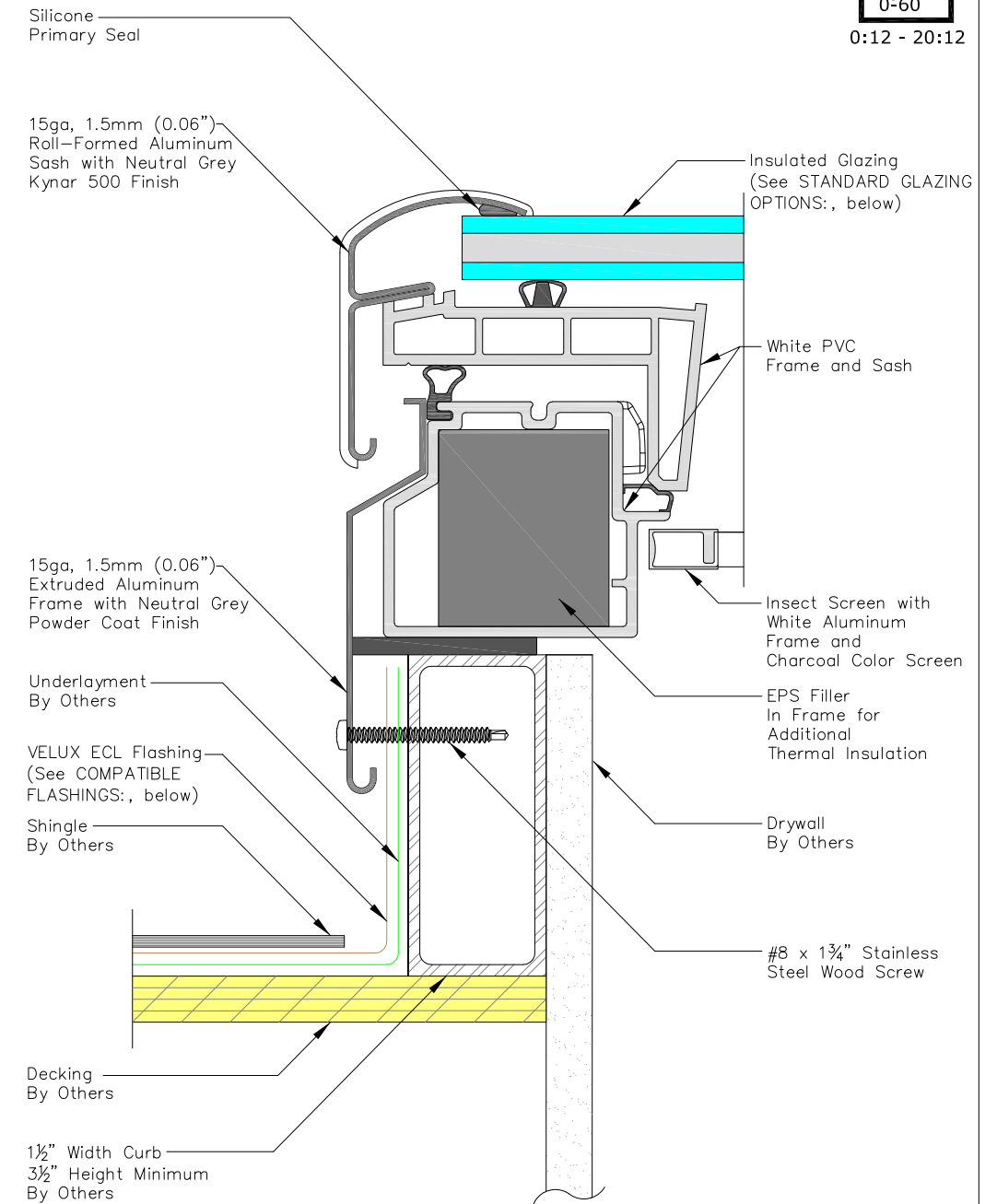
DETAIL 1
