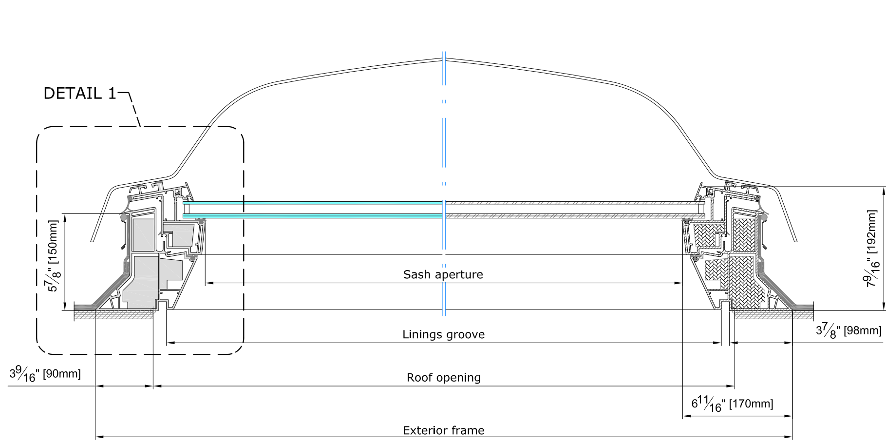
CROSS SECTION
