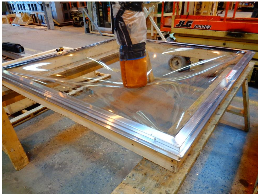
Photo No. 2 View of Tested Specimen with 400 lbs Applied
