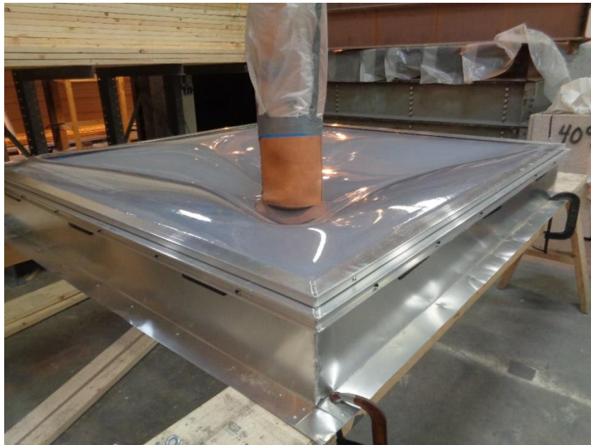
Photo No. 2 View of Tested Specimen with 400 lb Load Applied
