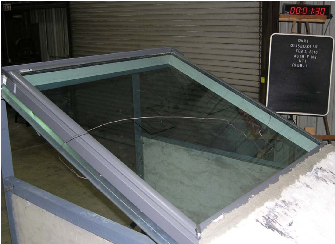
Figure B-1. Skylight prior to Start of Test.
