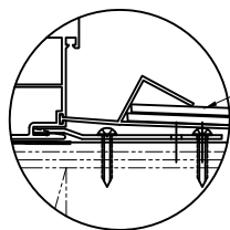
FLASHING LEG AT SIDE JAMB LOCATIONS ONLY
